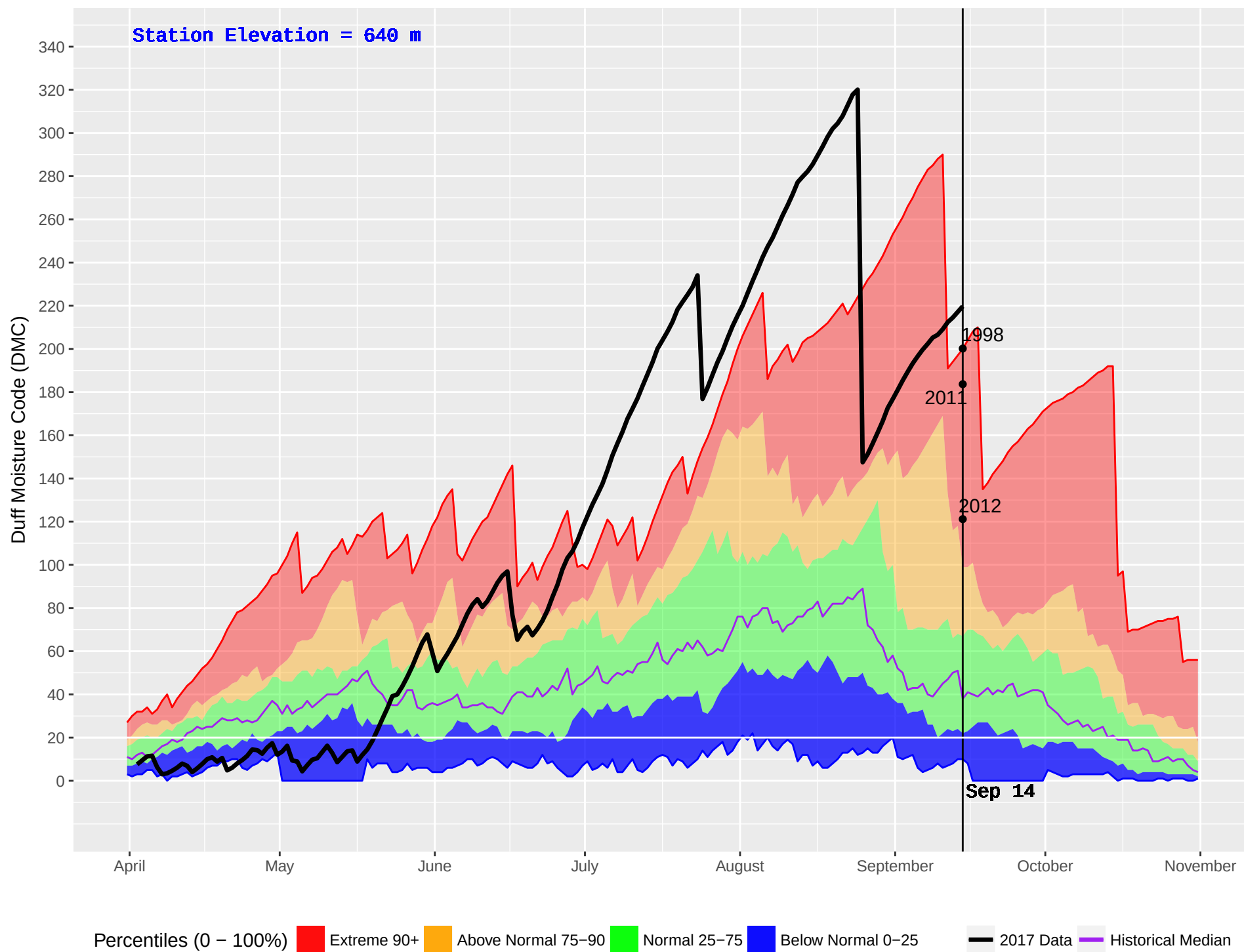
TURTLE (286) : Historical (1977–2016) and Current (2017) Noon Duff Moisture Code (DMC)
