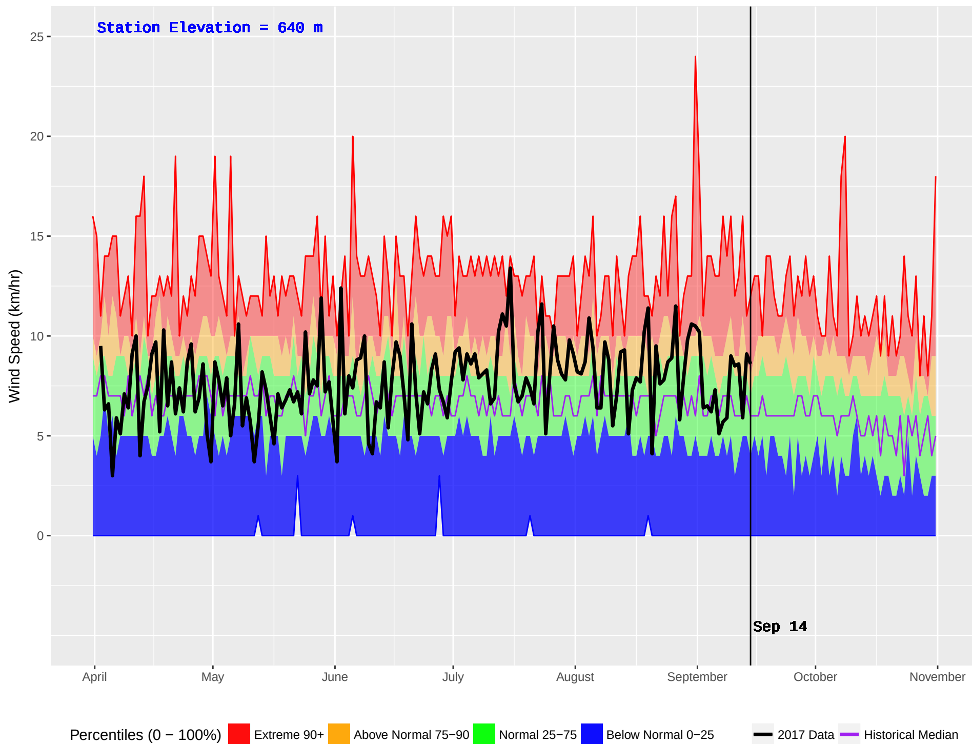
TURTLE (286) : Historical (1977–2016) and Current (2017) Noon Wind Speed
